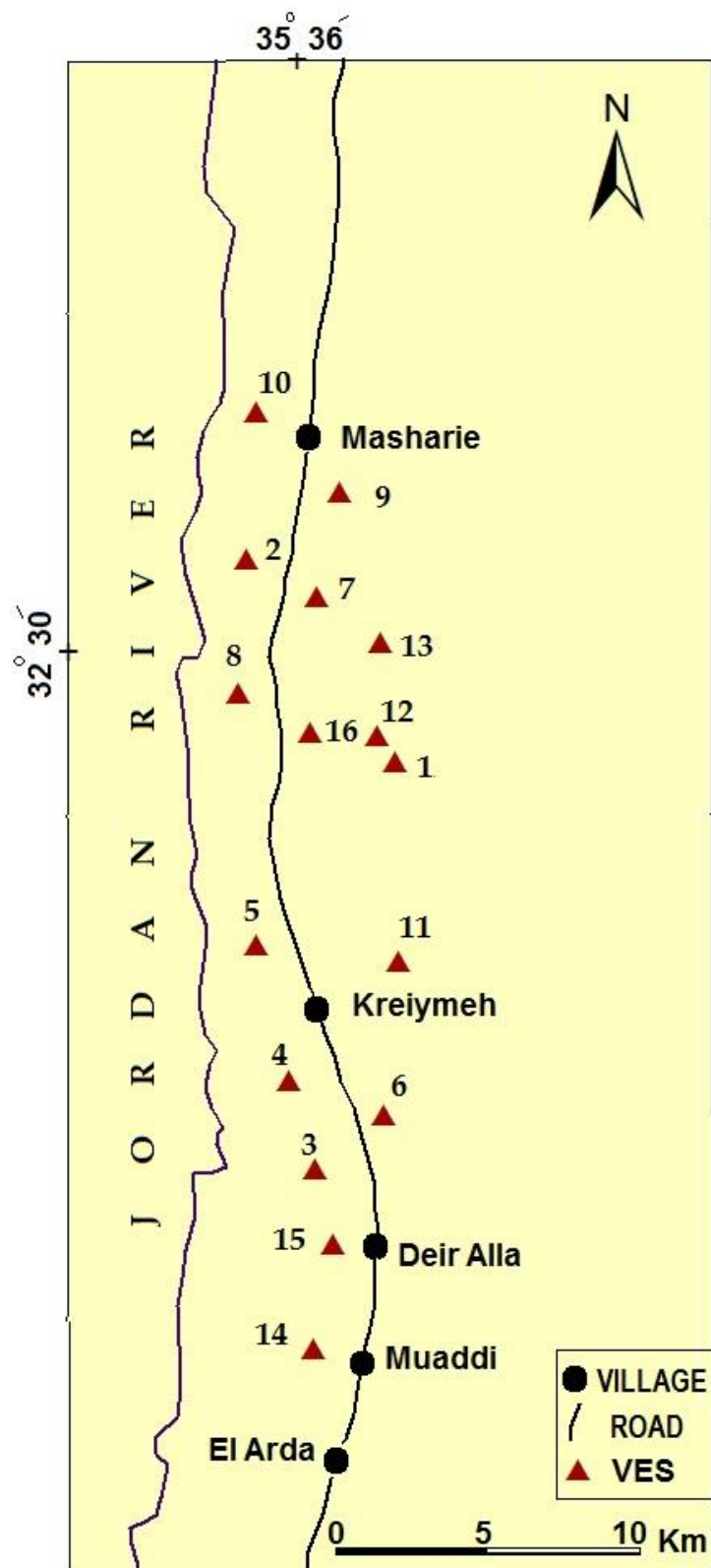
Fig (2) Vertical Electrical Sounding location map.
