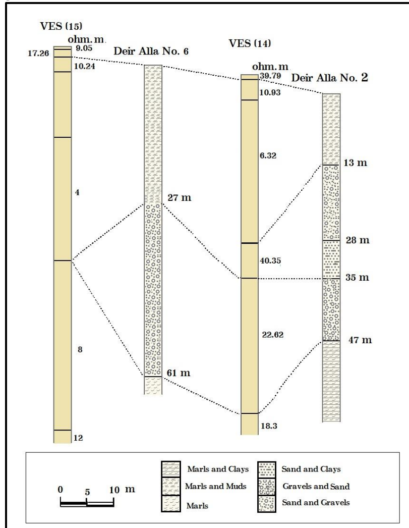
Fig (3) Correlation between [VES (14) and VES 15] to [wells log NO.2 and NO.6] both in Deir Alla area.
