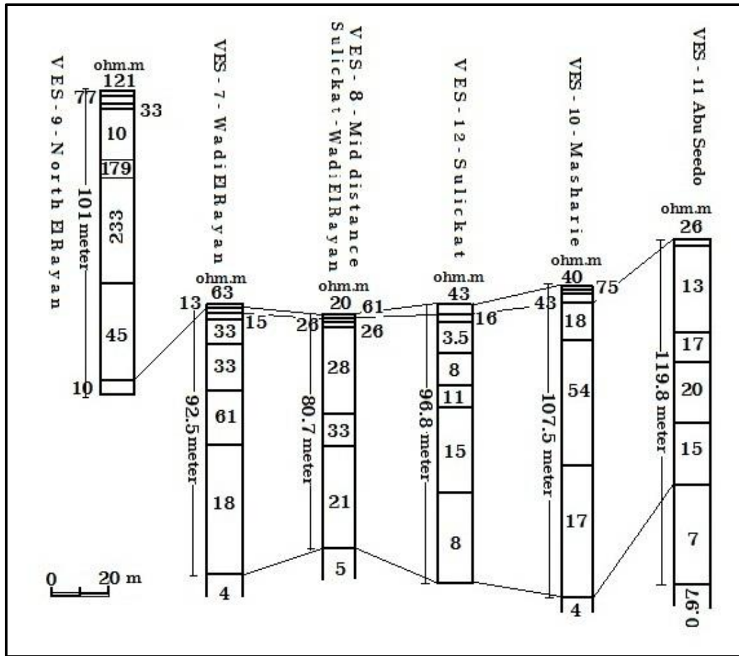
Fig (4) General correlation of resistivity interpreted data along the main road in the study area.
